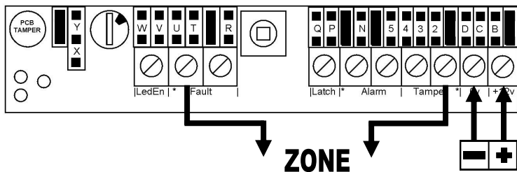
Example: G3 'Triple EOL/TEOL' Circuit (1k/1k/3k)
